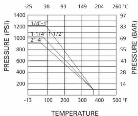
PRESSURE-TEMPERATURE RATING
